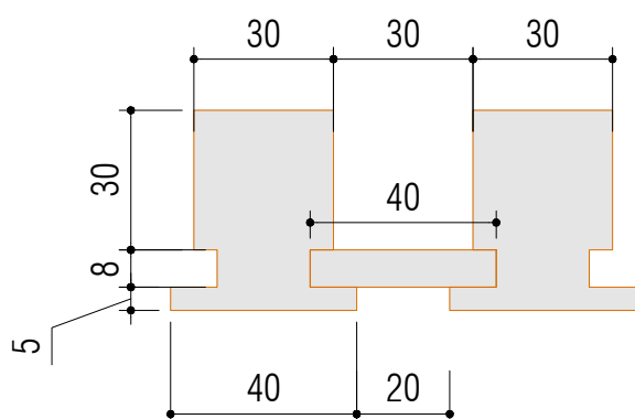
TASSEAUX BOIS- COUPE
